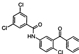
Compound # 51
